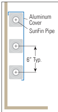
Tiered Installation
