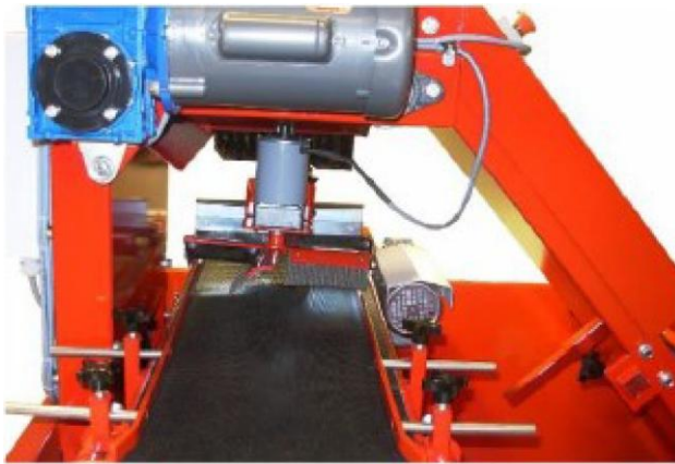
Adjustable Sweeper
